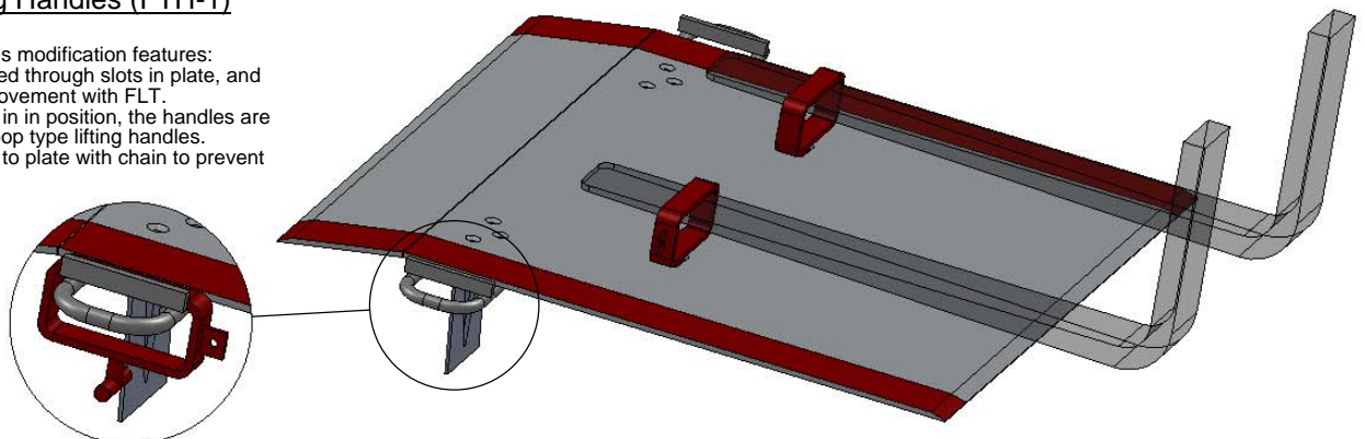
Handle in stored position.
